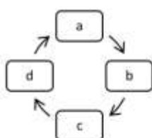
Directed Graph
