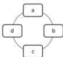
Undirected Graph
